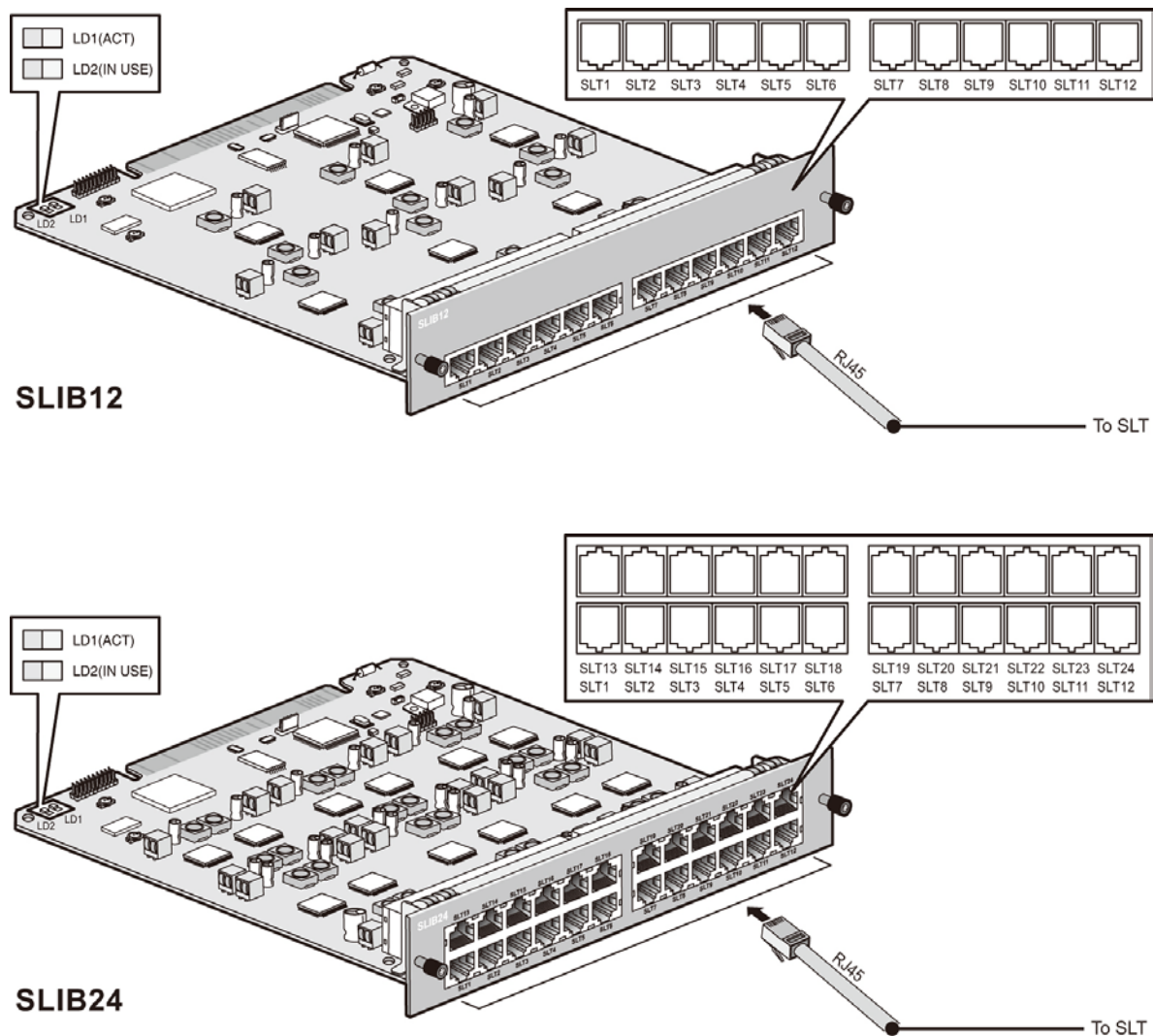
Figure 5.4.1-1 SLIB12/24
