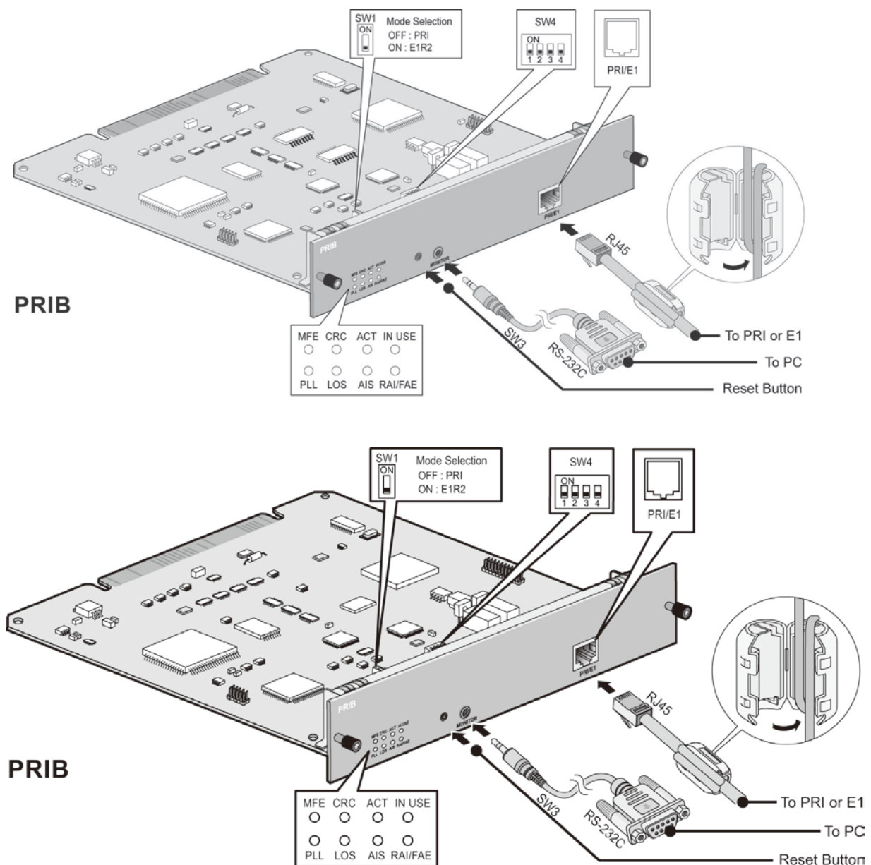
Figure 5.3.3-1 E1-PRIB
