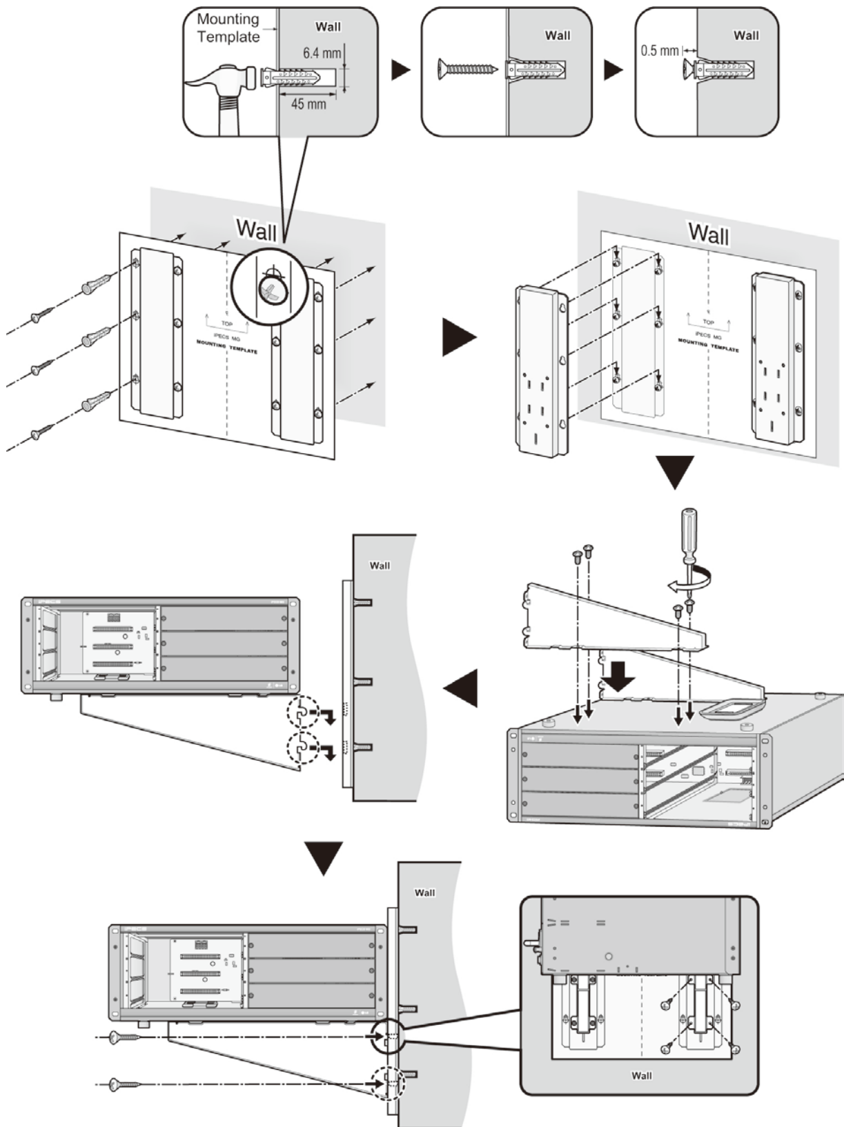
Figure 4.4.2-1 Wall Mounting
