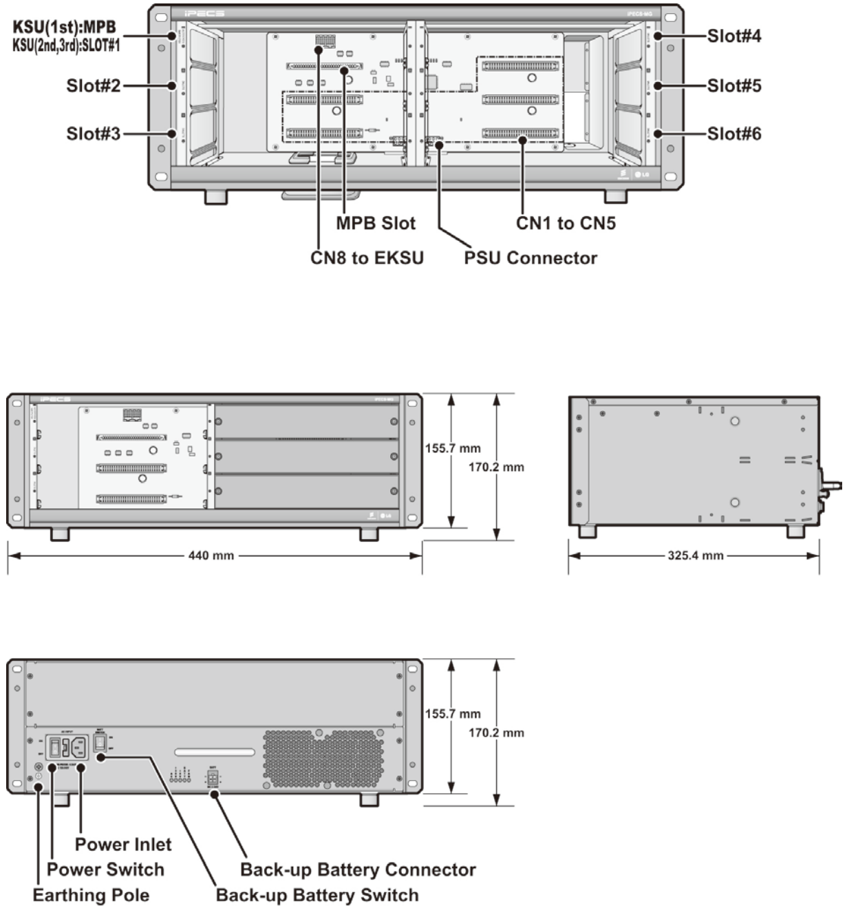
Figure 4.3-1 KSU Exterior and Dimension
