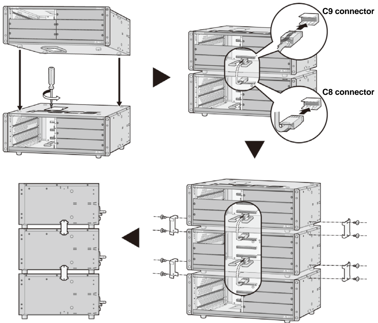
Figure 4.5-1 Expansion KSU installation
