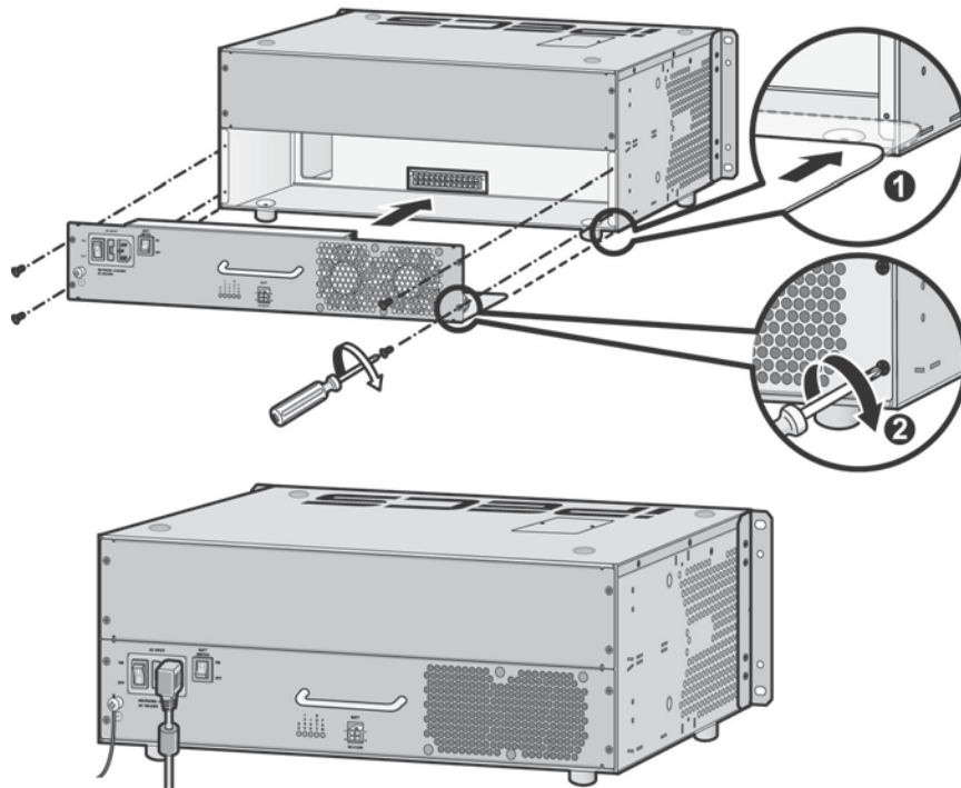
Figure 4.6.3-1 PSU Installation
