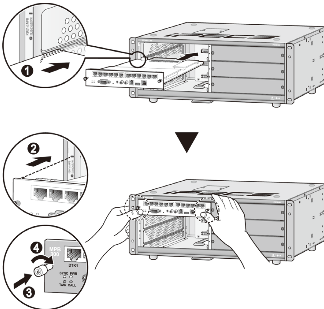
Figure 5.1-1 Board Installation
