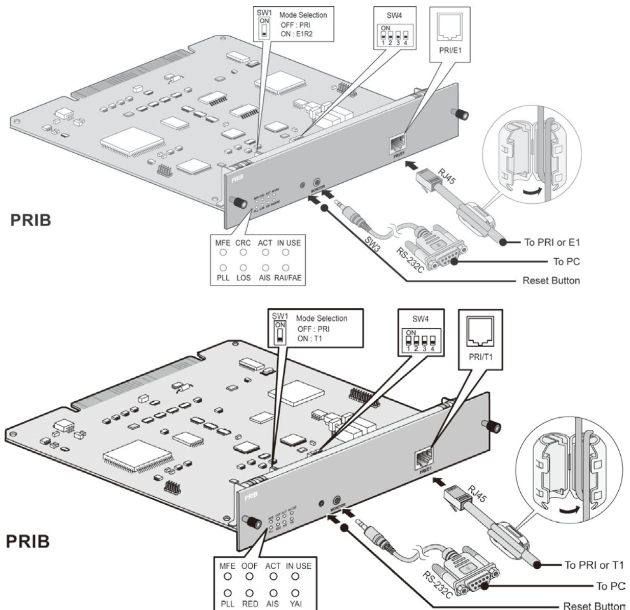
Figure 5.3.4-1 T1 PRIB
