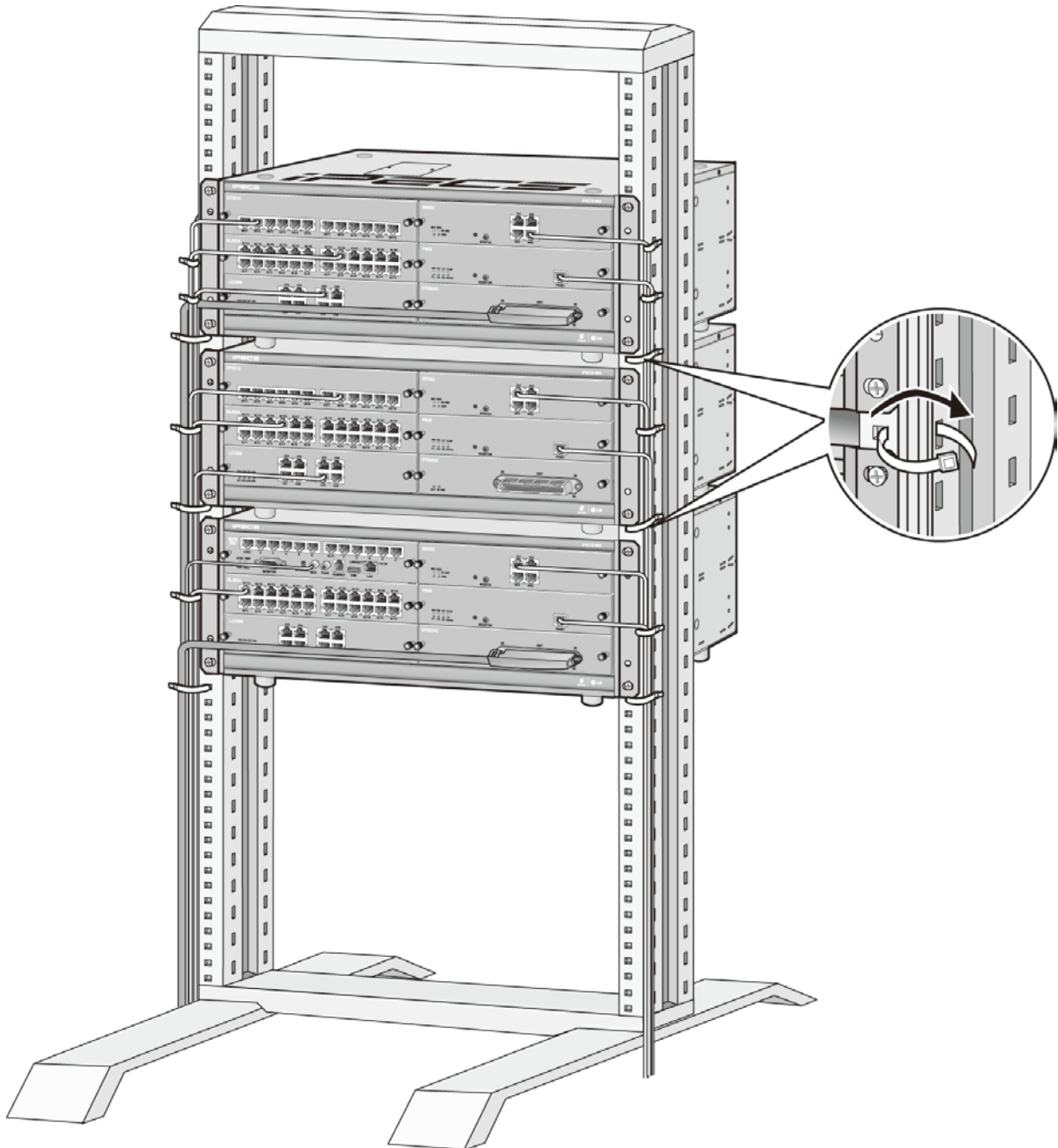
Figure 5.7.2-1 Rack Mount Cable Dressing
