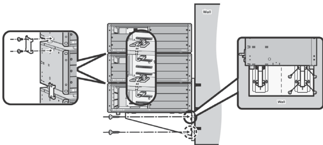
Figure4.5-2 Expansion KSU Wall Mounting
