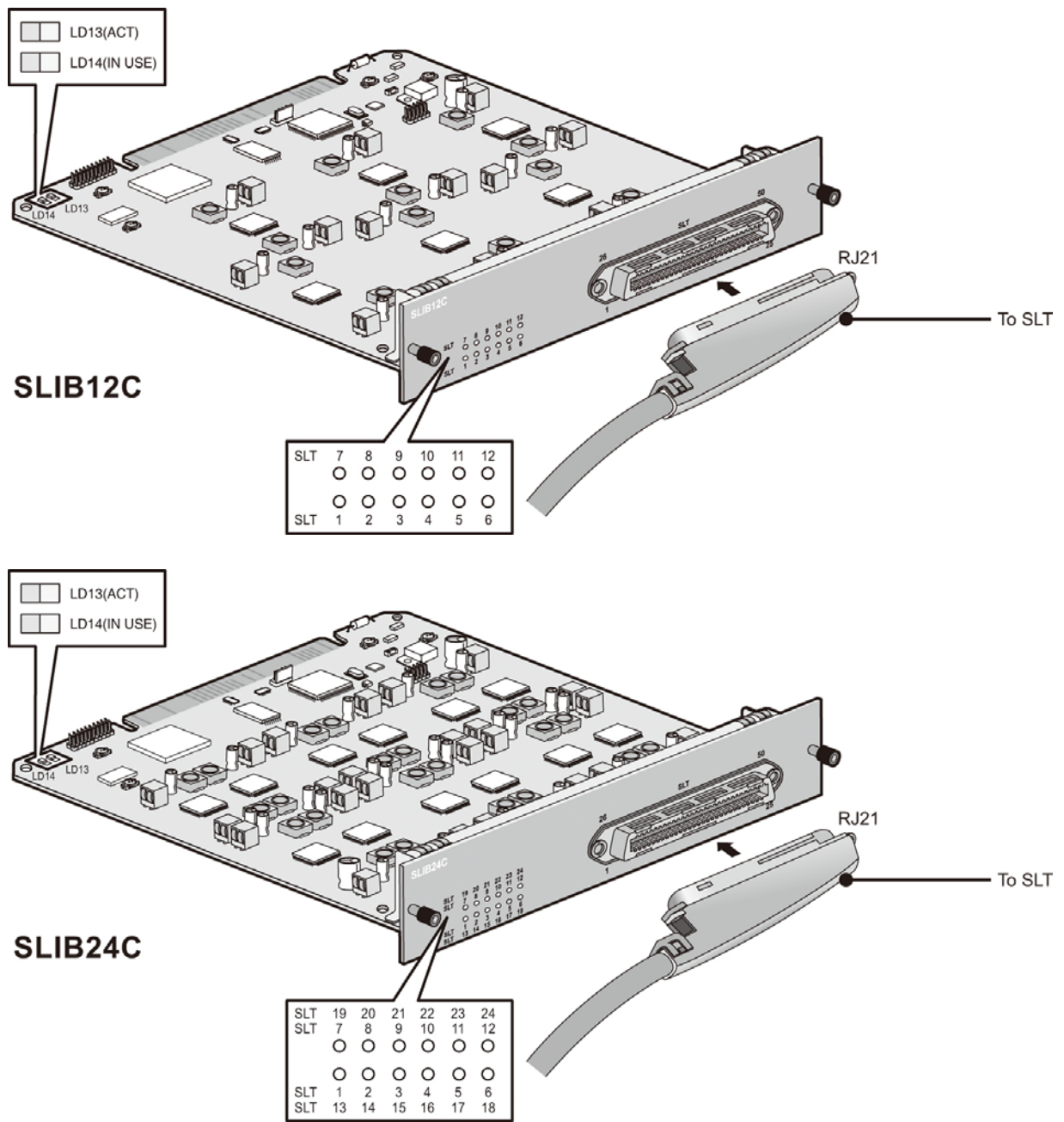
Figure 5.4.2-1 SLIB12/24C
