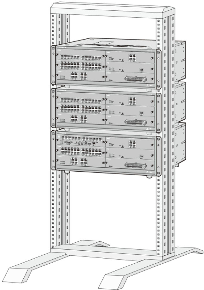
Figure 4.5-3 Expansion KSU Rack Mounting
