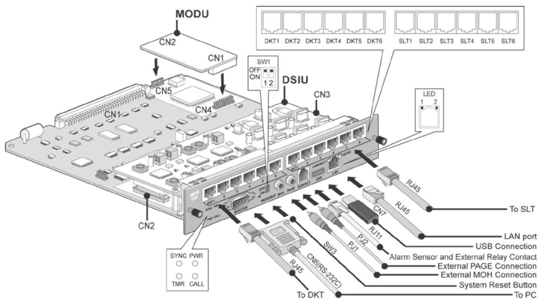
Figure 5.2-1 MPB
