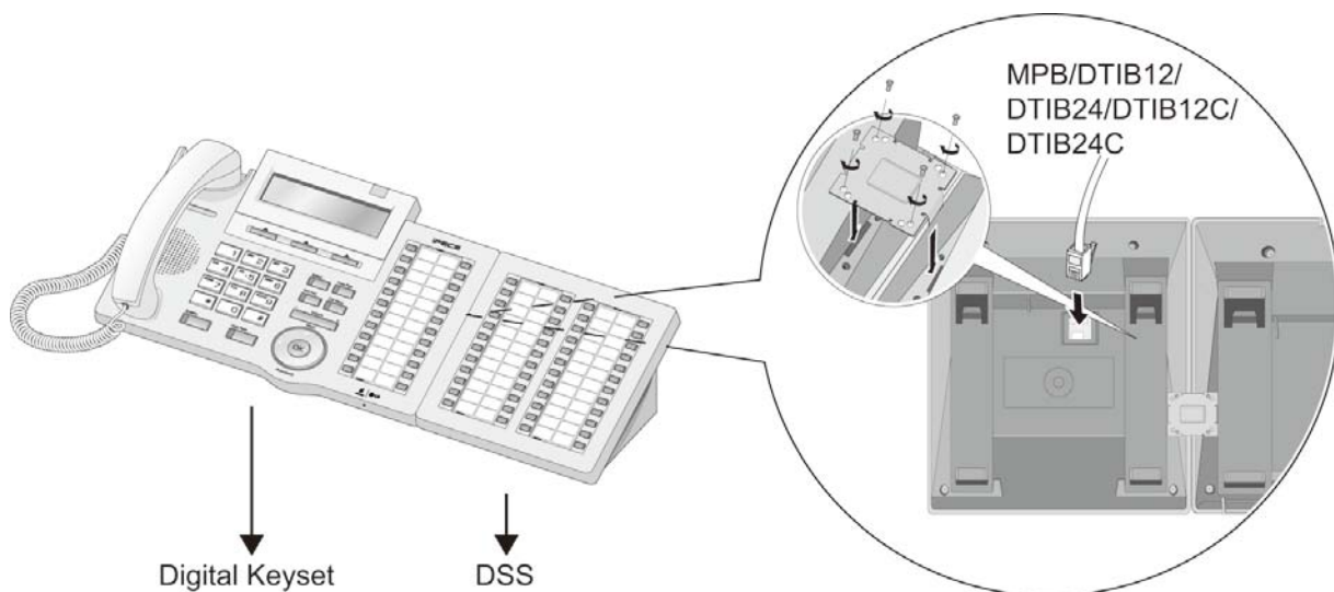
Figure 6.1.4.1-1 LDP-7048 and LIP-7048 Console Install
