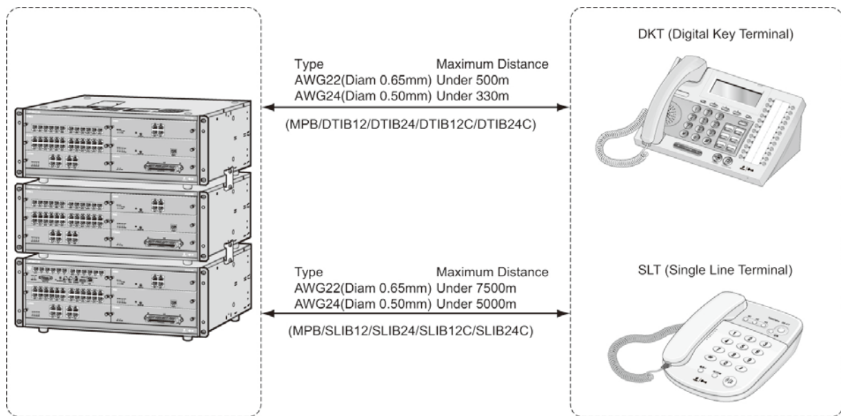
Figure 6.1.1-1 Terminal Cabling Distance
