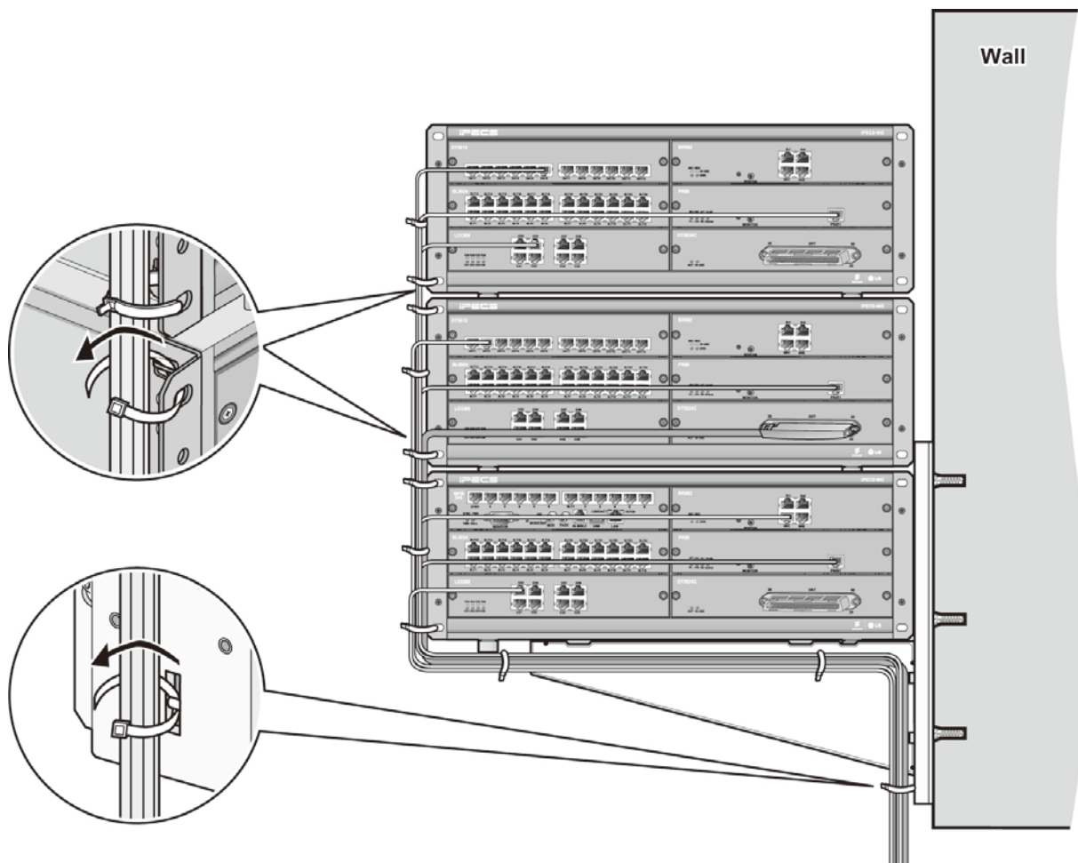
Figure 5.7.1-1 Wall Mount Wiring
