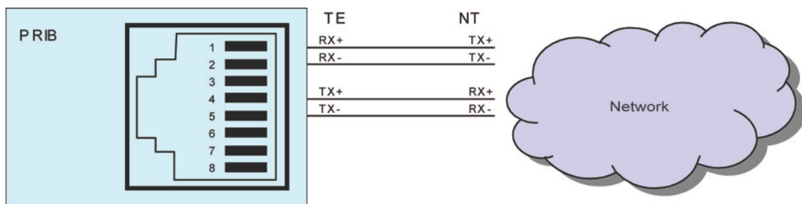
Figure 5.3.3.3-1 E1-PRIB Connector Wiring Diagram
