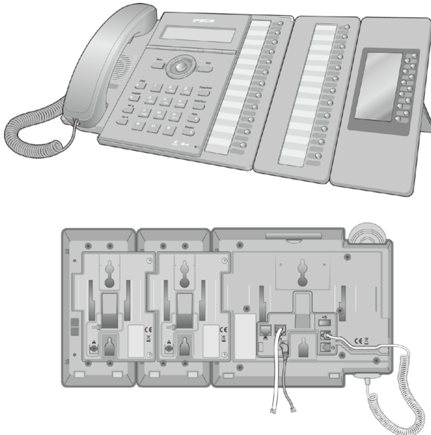
Figure 6.1.4-2 LIP-8000 DSS Installation (12DSS + 12LSS)
