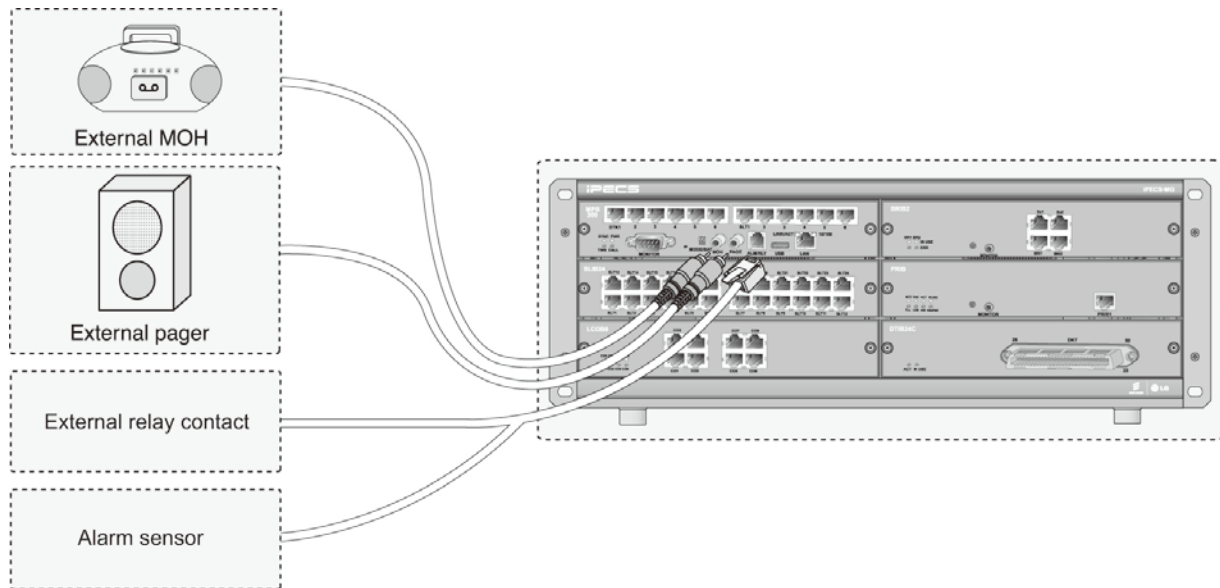
Figure 5.2.5-1 Miscellaneous Connections
