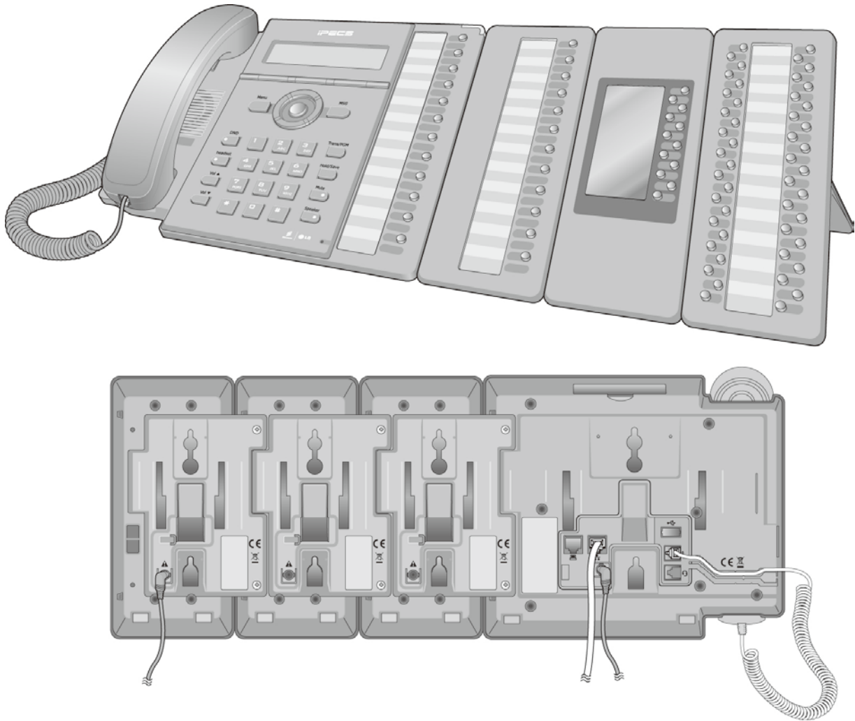
Figure 6.1.4-3 LIP-8000 DSS Installation (12DSS + 12LSS+48DSS)
